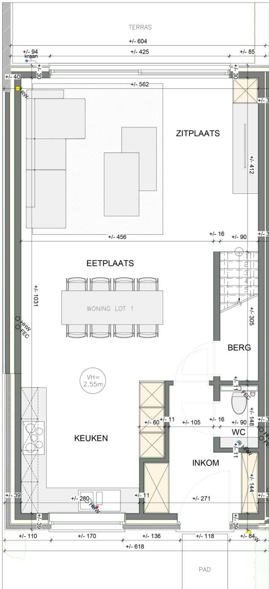
N+00 (1/50)
