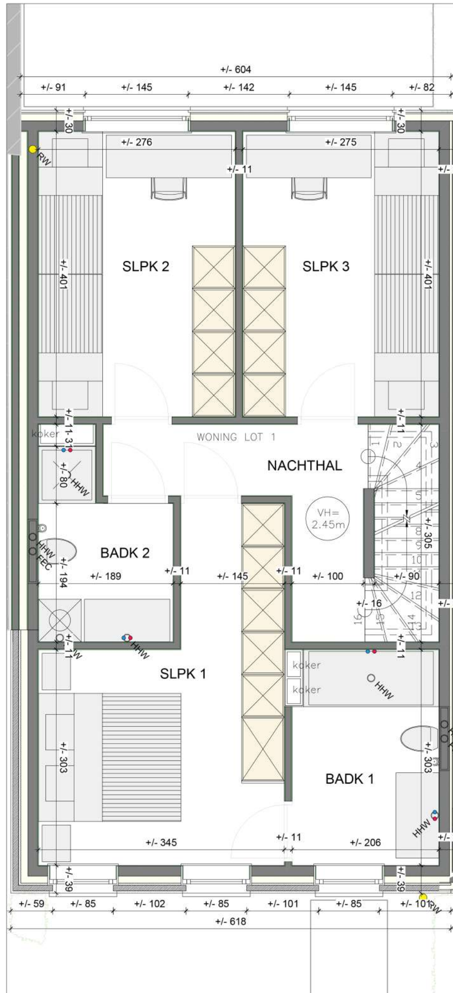
N+01 (1/50)
